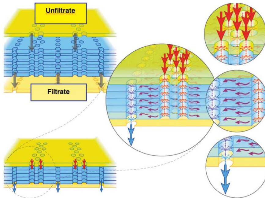
Figure 1: SUPRApak flow configuration
